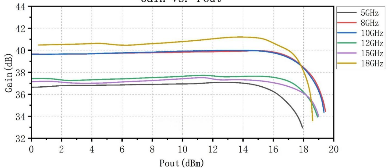
Gain VS. Pout
