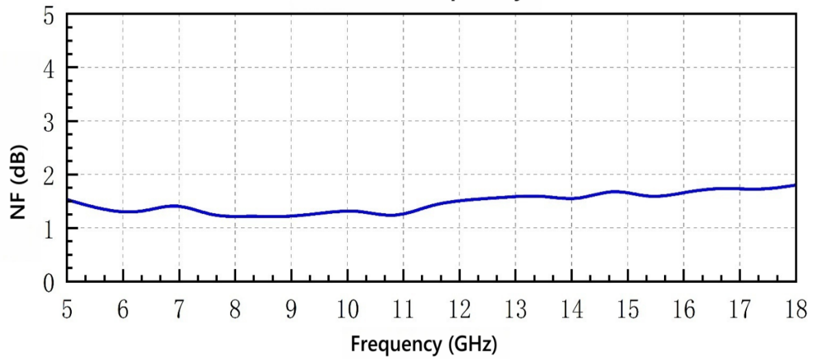
NF VS Frequency
