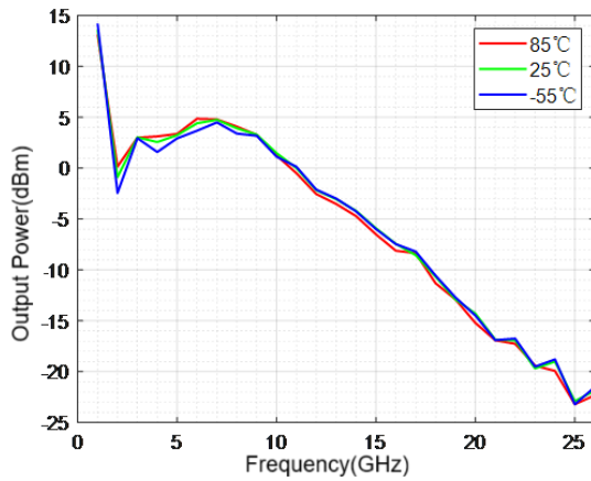
Output Power (VCC=5V, Input power 0dBm)
