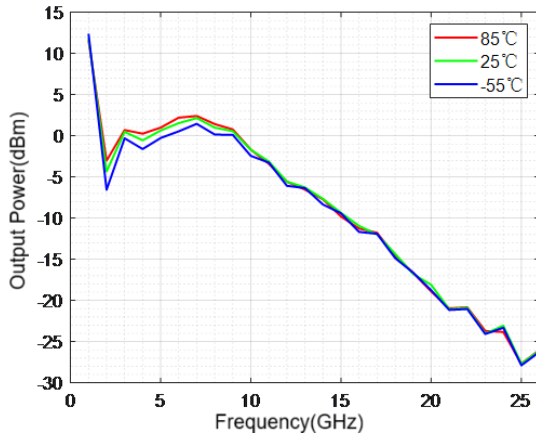
Output Power (VCC=4.5V, Input power 10dBm)
