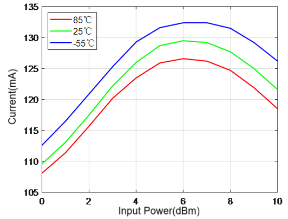
Current (VCC=5V)
