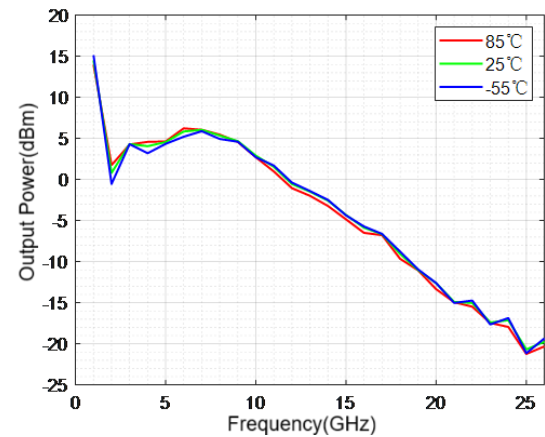
Output Power (VCC=5V, Input power 5dBm)
